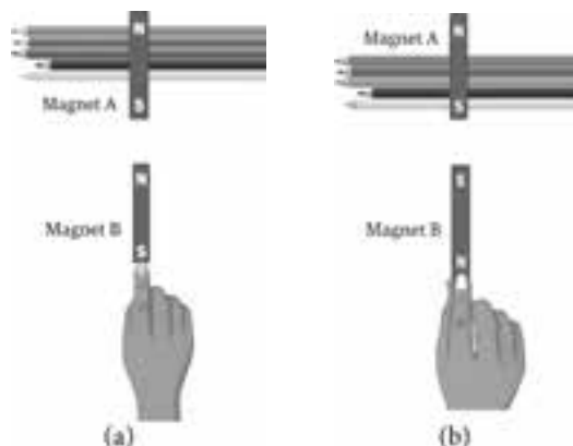
Figure : Interaction between two bar magnets
