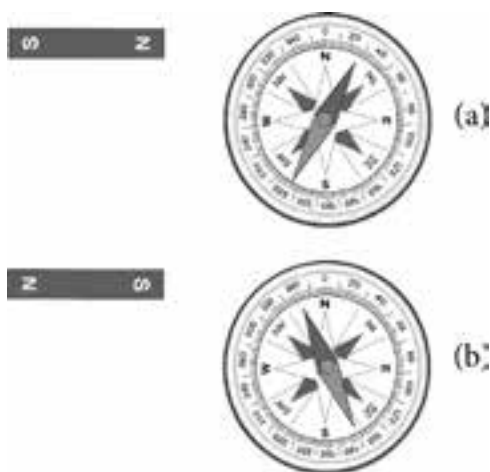
Figure : A compass needle and a magnet
