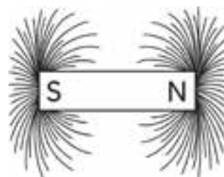
Figure : Iron filings sticking to a bar magnet
