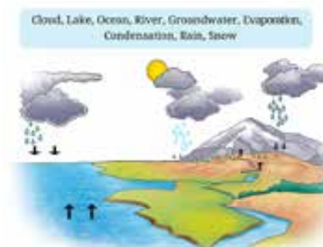
Figure : Change of states and movement of water
