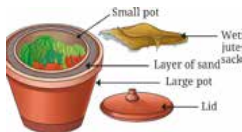
Figure : A pot-in-pot cooler
